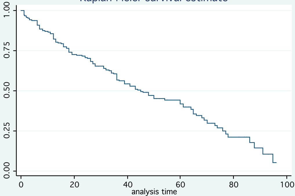
Kaplan-Meier survival estimate
