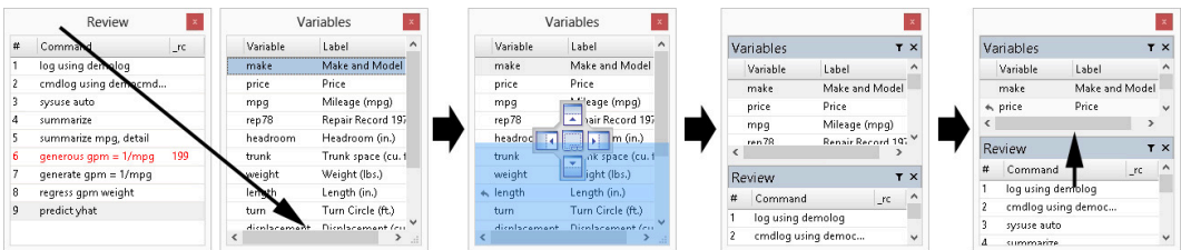
Figure 1: Linking two windows
